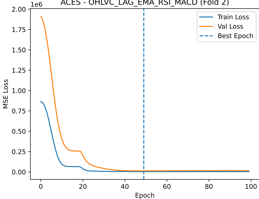
ACES - OHLVC_LAG_EMA_RSI_MACD (Fold 2)
